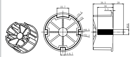
1.0405.0101 Bouchon (Axe round)
