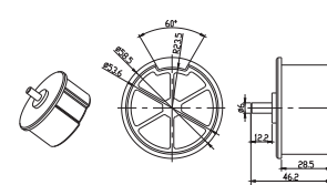
1.0404.0072 Bouchon (Axe round)
